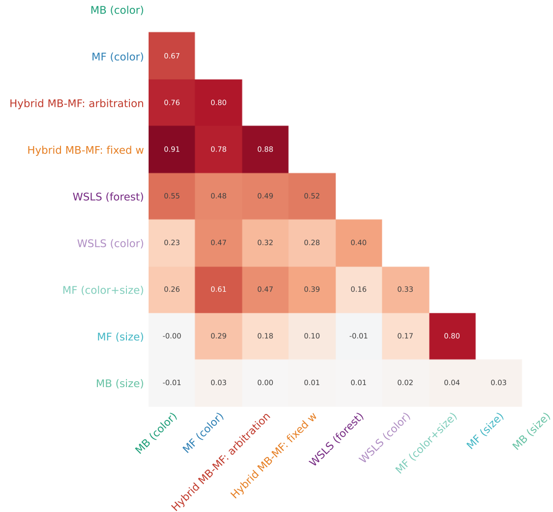
Choice probability similarity
