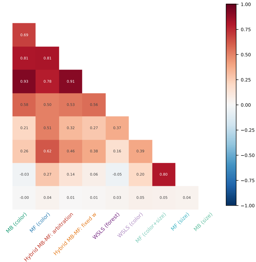
Corrected reward similarity
